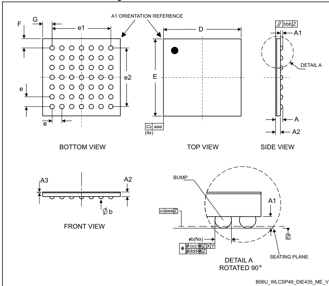
Figure 56. WLCSP49 - Outline
