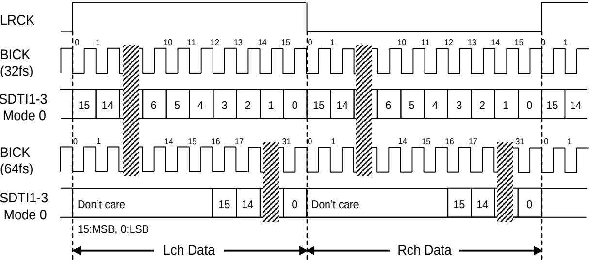
Figure 18. Mode 0 Timing
