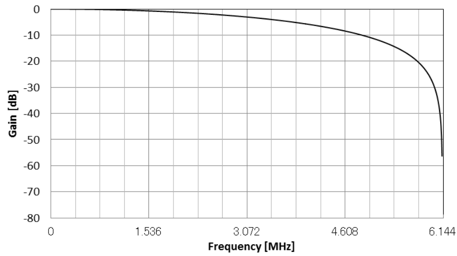
Figure 62. Mode7 FIR Filter (Except DSD Direct Mode)
