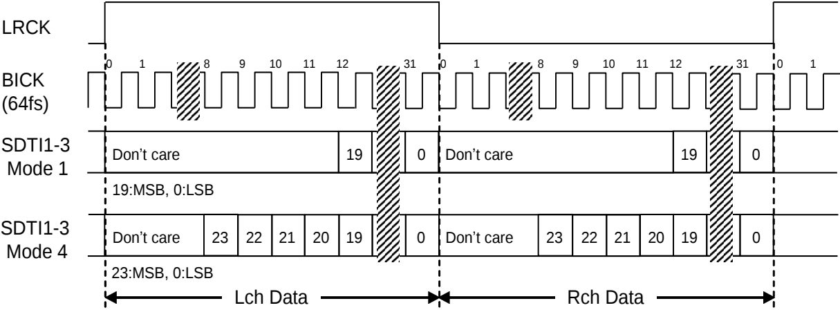
Figure 19. Mode 1/4 Timing
