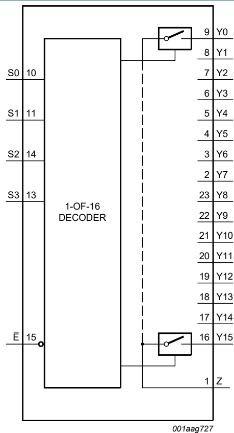
Fig. 4. Functional diagram
