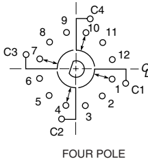
FOUR POLE
