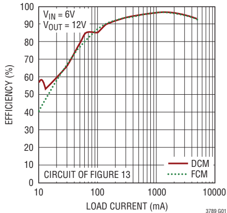
Efficiency vs Output Current (Boost Region)
