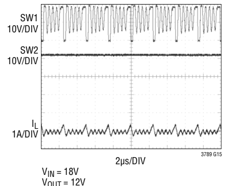
Pulse-Skipping Mode
