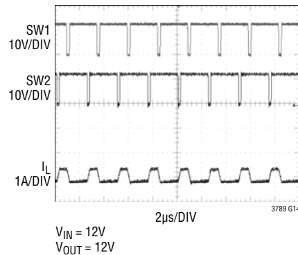
Pulse-Skipping Mode
