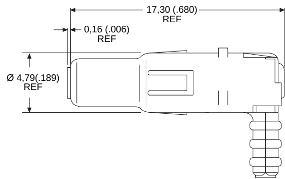
Plug
