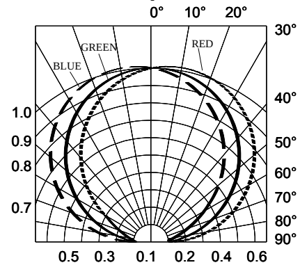
Radiation Diagram
