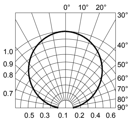
Radiation Diagram
