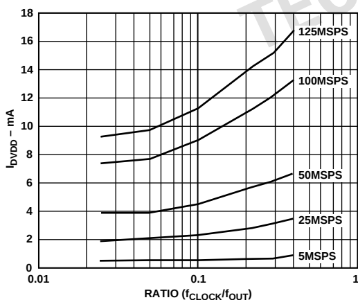
Figure 29. I_{DVDD} vs. Ratio @ DVDD = 5 V
