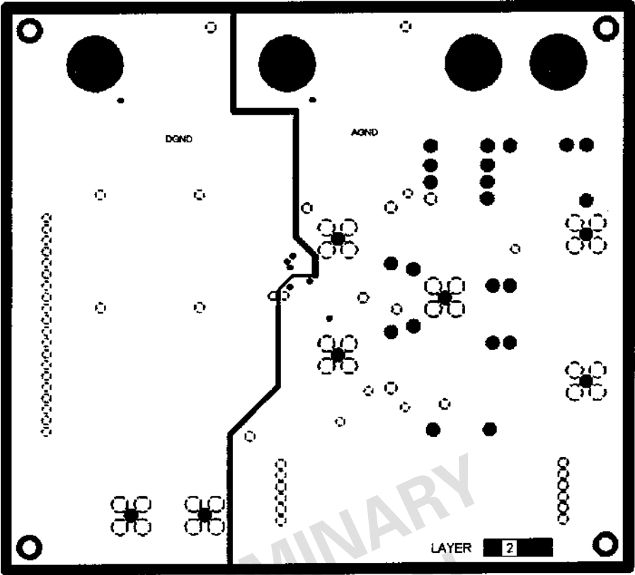
Figure 42. Ground Plane PCB Layout (Layer 2)
