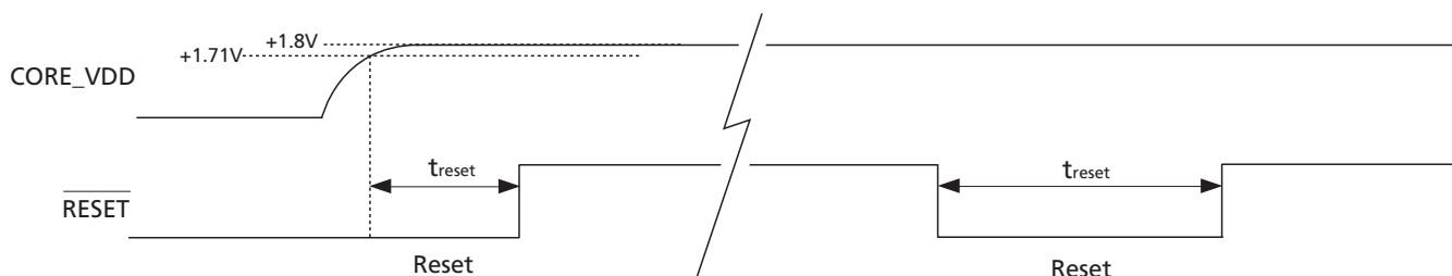
Figure 3-19: Reset pulse
