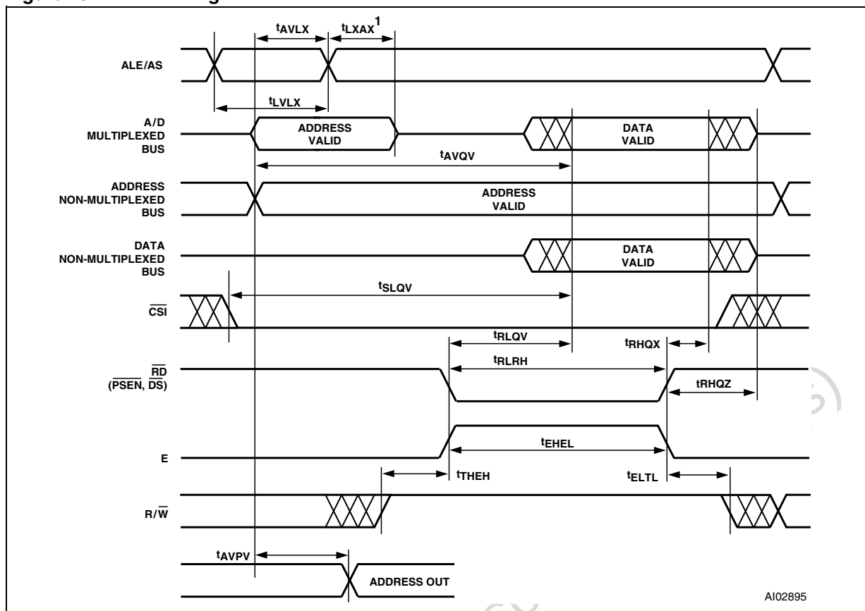
Figure 45. READ Timing
