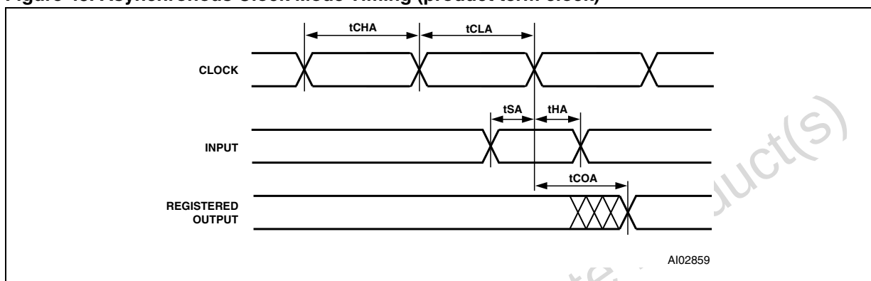
Figure 43. Asynchronous Clock Mode Timing (product term clock)
