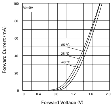
Clamp Diode Forward Current vs. Voltage
