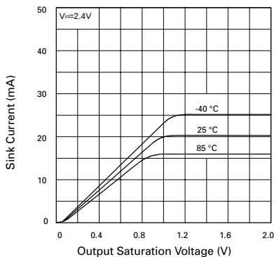
Output Saturation Voltage vs. Sink Current
