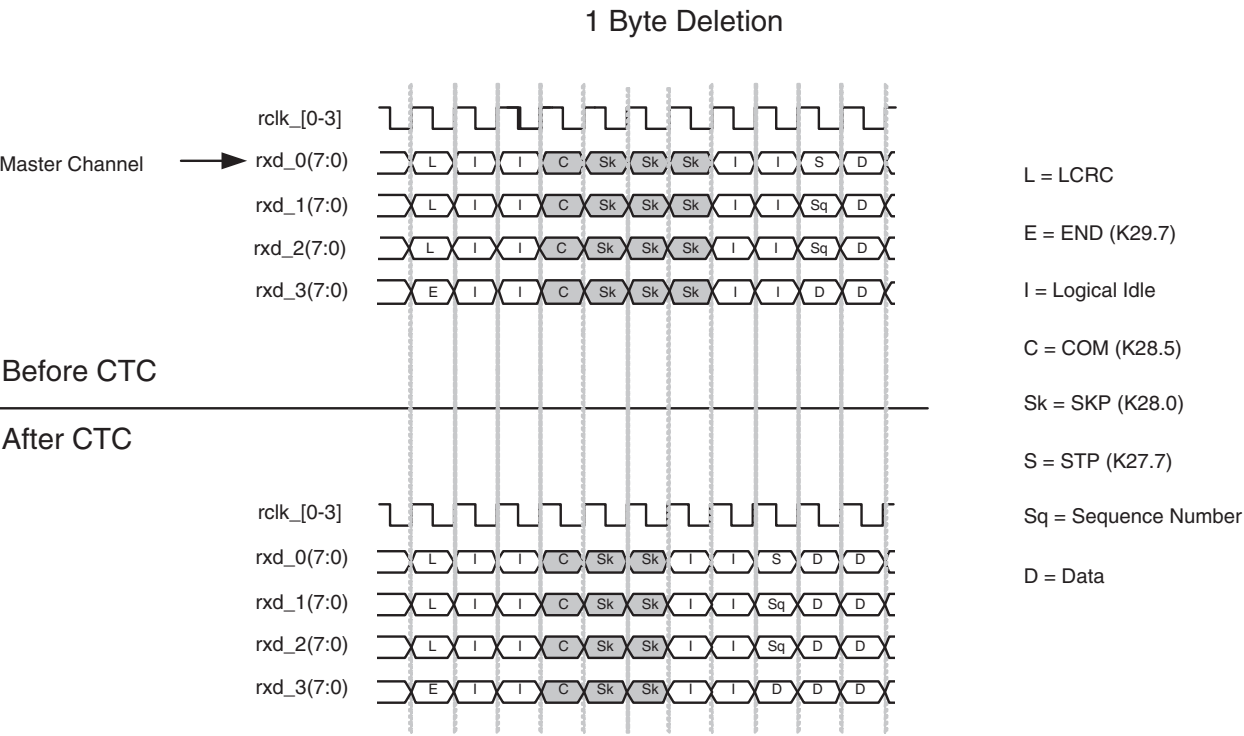
Figure 8-13. x4 PCI Express Operation Clock Compensation Byte Deletion Example
