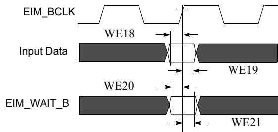
Figure 13. EIM Inputs Timing Diagram
