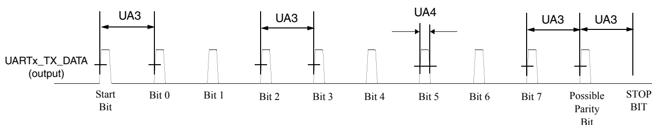
Figure 102. UART IrDA Mode Transmit Timing Diagram
