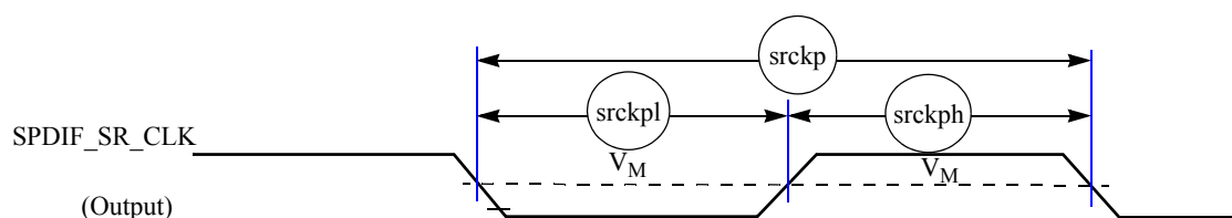
Figure 94. SPDIF_SR_CLK Timing Diagram
