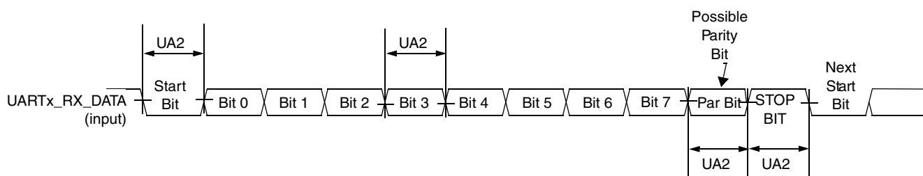
Figure 101. UART RS-232 Serial Mode Receive Timing Diagram
