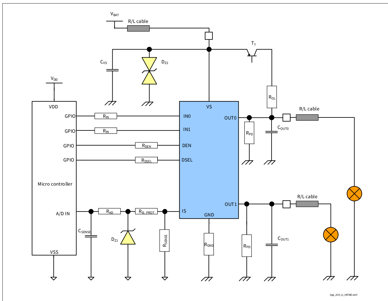
Figure 43 BTS7012-2EPA Application Diagram
