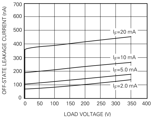
Figure 10. Leakage Current vs. Applied Voltage at 70°C
