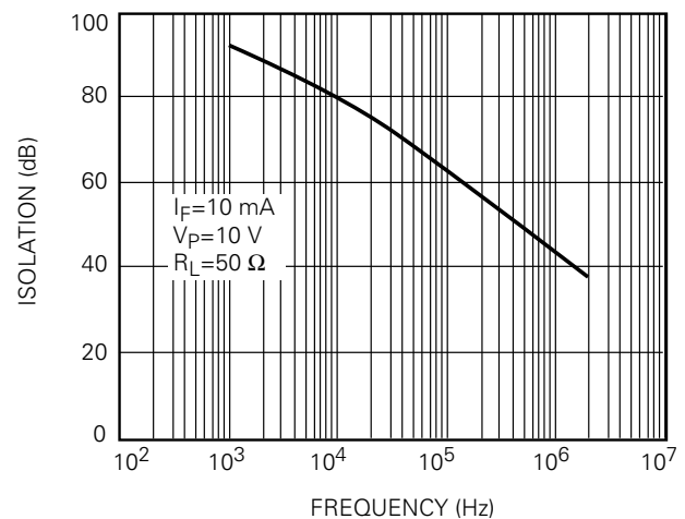
Figure 6. Output Isolation
