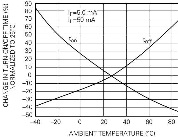
Figure 14. Turn-on/off Time vs. Temperature
