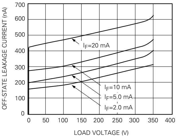
Figure 11. Leakage Current vs. Applied Voltage at 85°C
