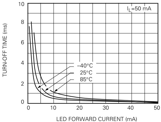
Figure 16. Turn-off Time vs. LED Current
