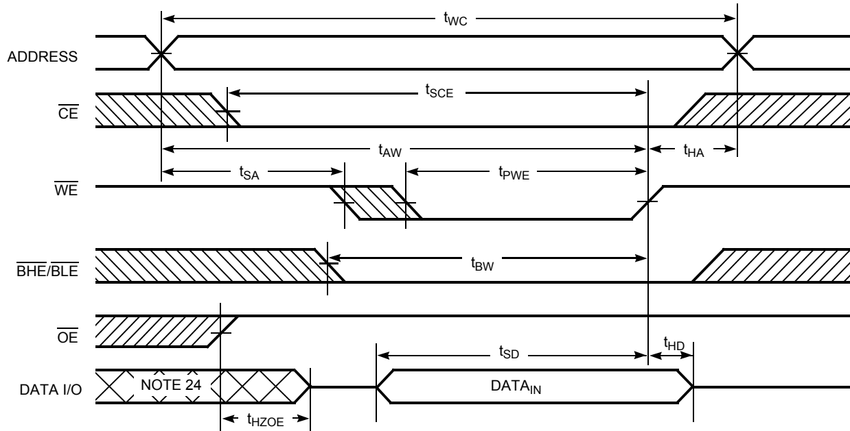
Figure 6. Write Cycle No. 2 ( \overline{\text{CE}} Controlled) [22, 23]
