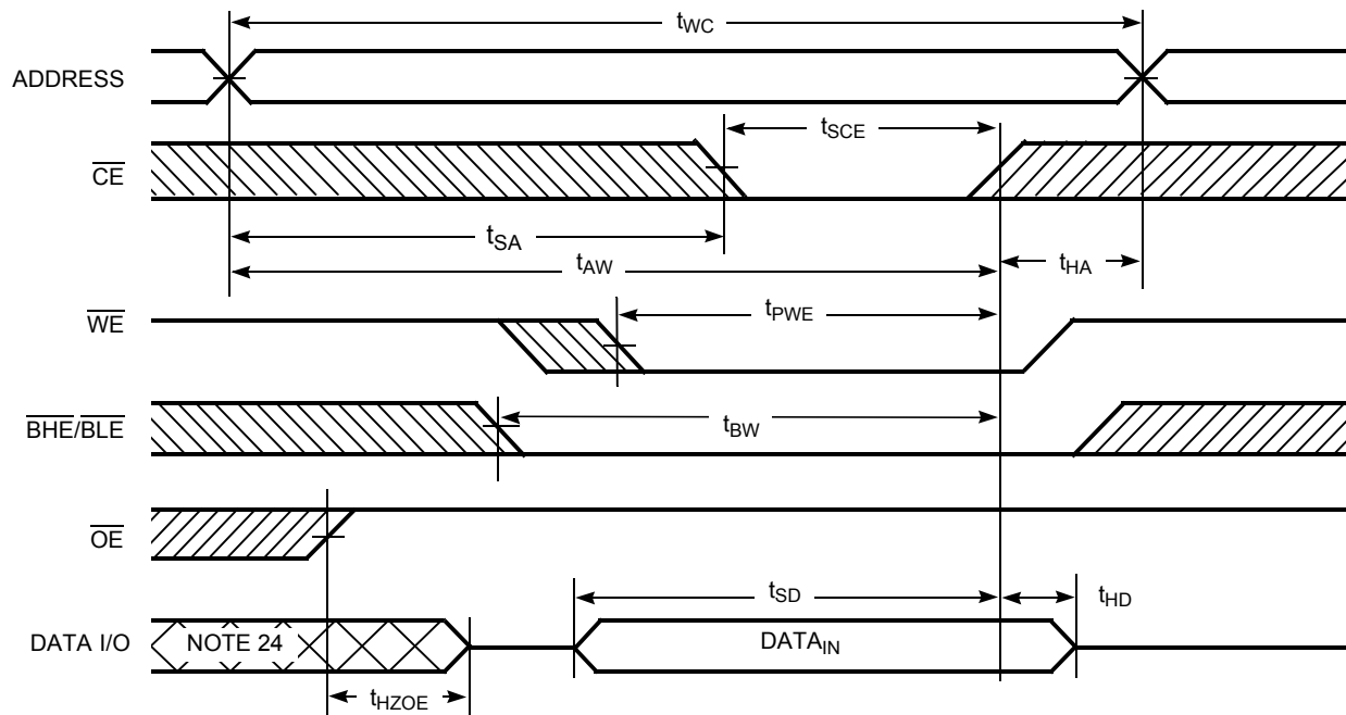
Figure 6. Write Cycle No. 2 ( \overline{\text{CE}} Controlled) [22, 23]
