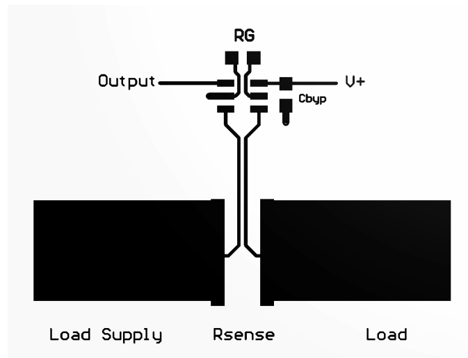
Figure 10-1. Layout Example
