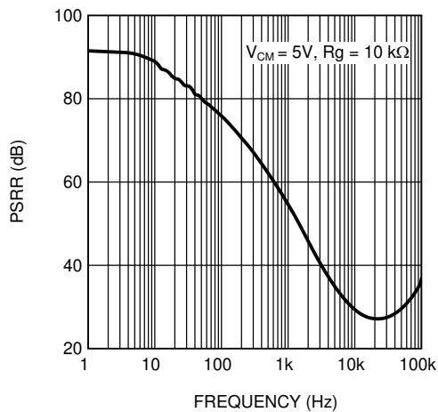
Figure 6-3. AC PSRR vs. Frequency
