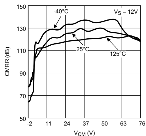
Figure 6-6. CMRR vs. V_{CM}
