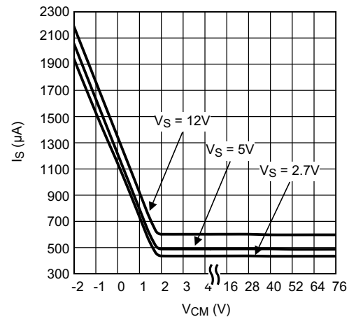
Figure 6-2. Supply Current vs. V_{CM}
