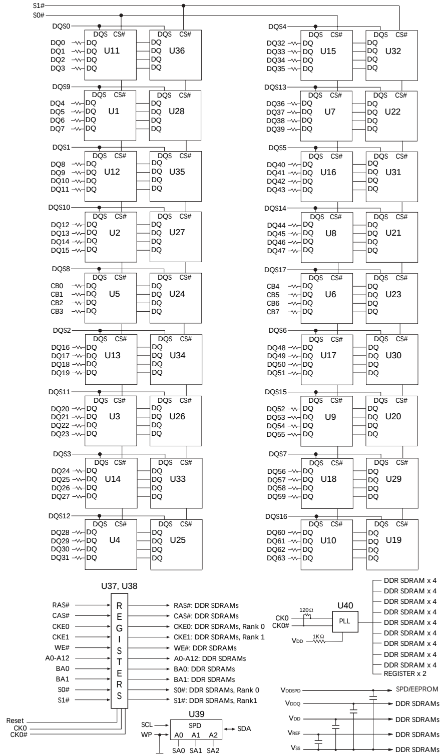
Figure 4: Standard PCB Functional Block Diagram – 1GB, 2GB
