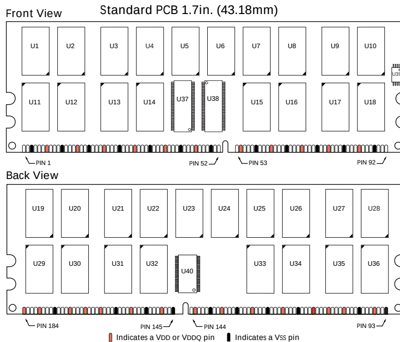
Figure 2: Pin Locations (Standard PCB)
