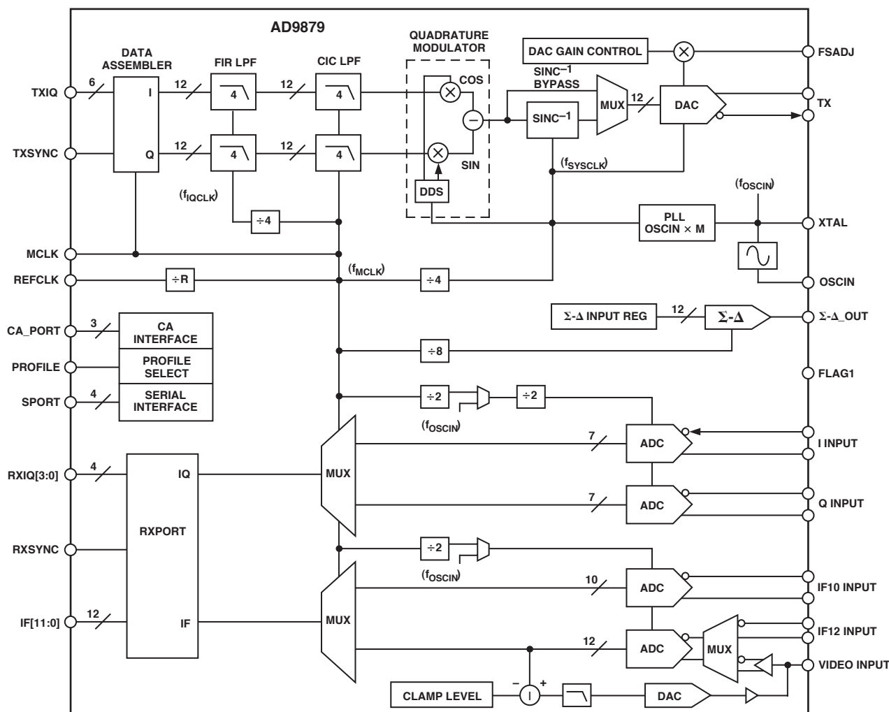
Figure 1. Block Diagram
