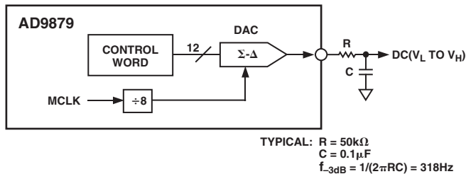
Figure 6. Sigma-Delta RC Filter
