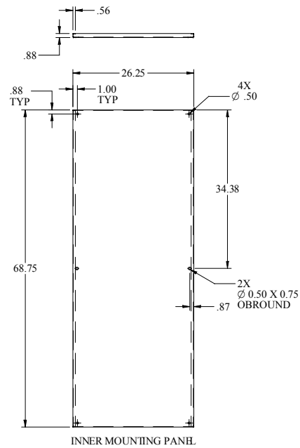
INNER MOUNTING PANEL
