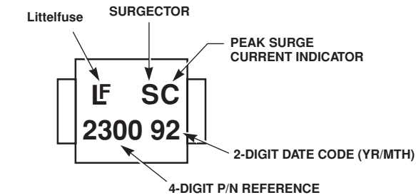
SGT2300SC (TOP VIEW - NOT TO SCALE)
