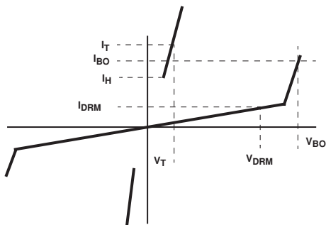
FIGURE 1. V-I CHARACTERISTICS
