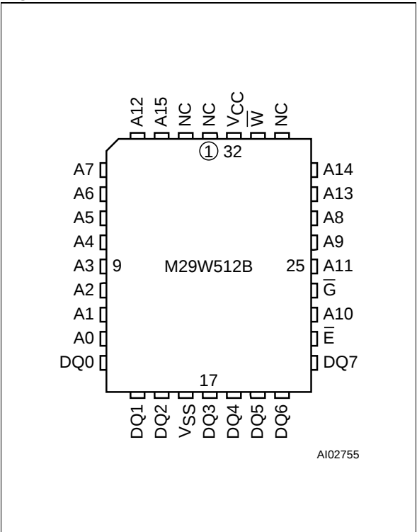
Figure 3. PLCC Connections
