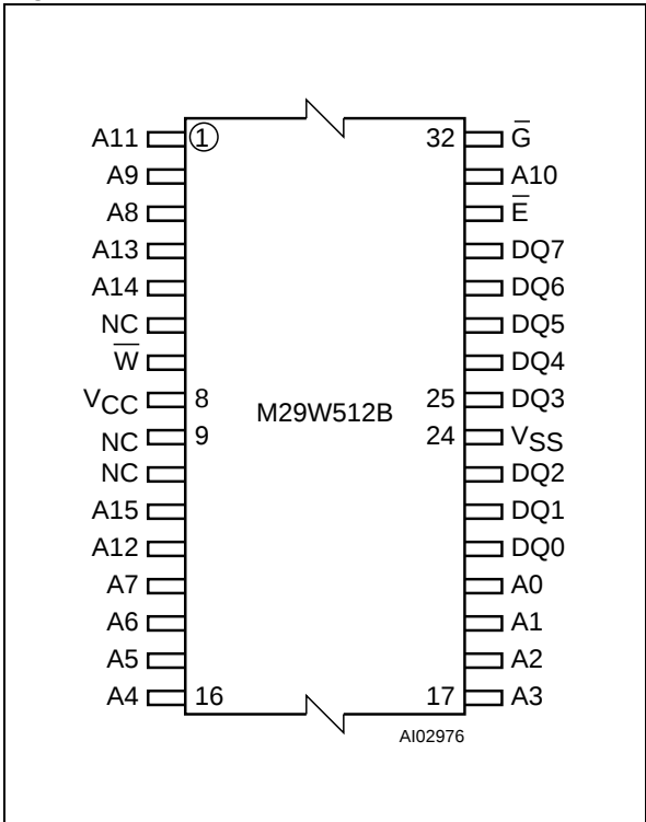
Figure 2. TSOP Connections
