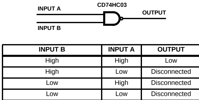
FIGURE 11C. CMOS OPEN DRAIN
