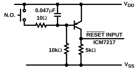
FIGURE 15. POWER ON RESET
