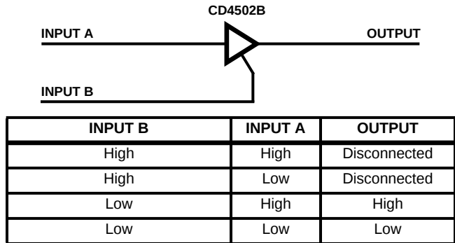
FIGURE 11D. CMOS TRI-STATE BUFFER
