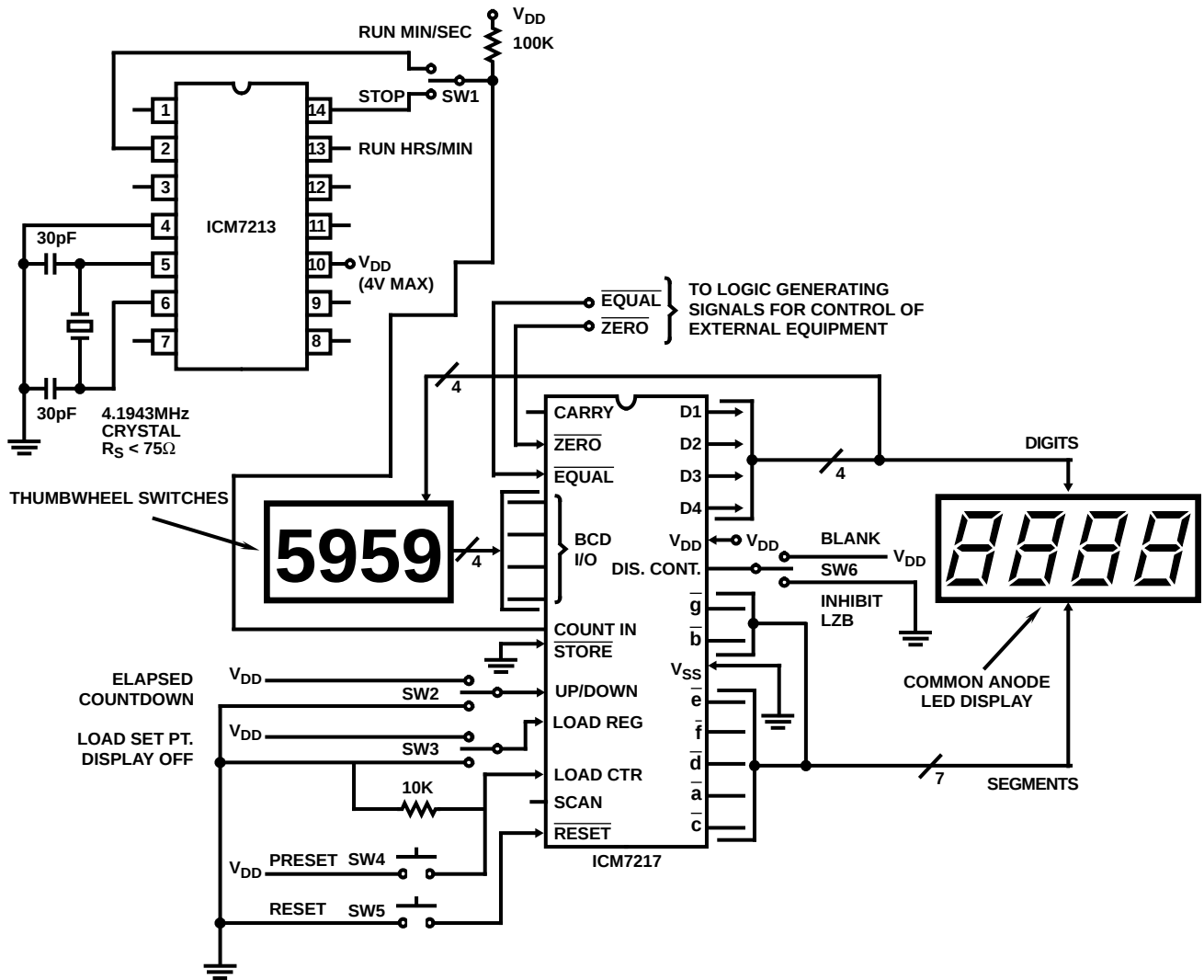
FIGURE 21. PRECISIONS TIMER
