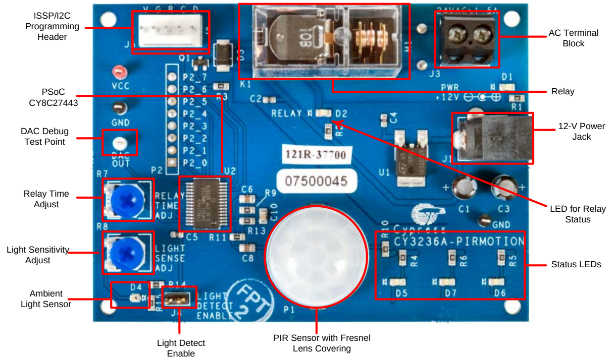
Figure 4-2. CY3236A-PIRMOTION Board
