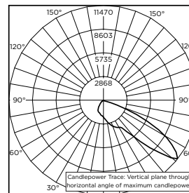
ITL Test Report #: 76042 BXSPA*GHA-U Initial Delivered Lumens: 11,092
