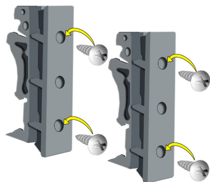
DIN-Rail Mounting Kit for 1&2 Port ES/UC
