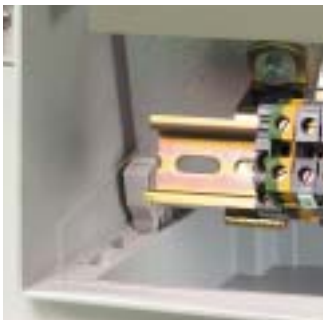
The base plate can be snap-mounted inside the switchboard.
