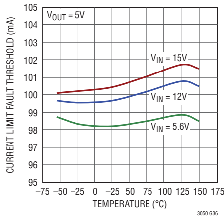
External Current Limit R_{I\text{MAX}} = 1.15k
