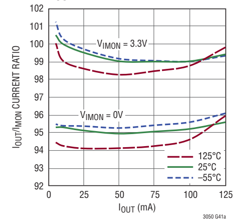
I_{\text{OUT}}/I_{\text{MON}} Current Ratio V_{\text{OUT}} = 3.3V , V_{\text{IN}} = 3.9V
