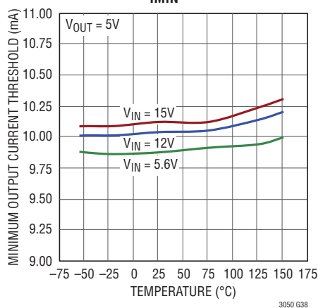
Minimum Output Current Threshold R_{I\text{MIN}} = 11.3k
