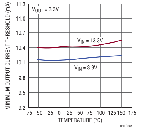
Minimum Output Current Threshold R_{I\text{MIN}} = 11.3k
