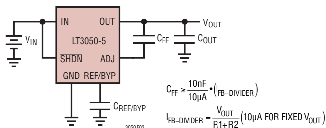
Figure 2. Feedforward Capacitor for Fast Transient Response
