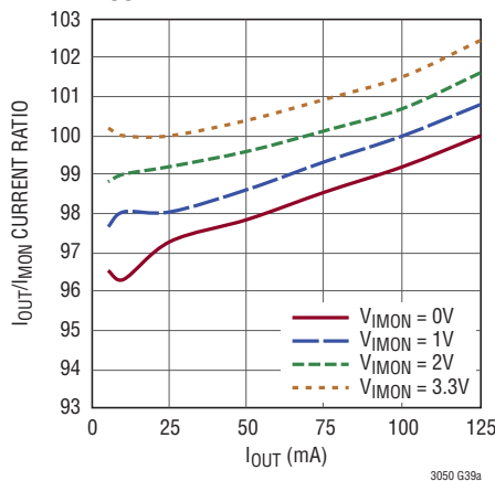
I_{\text{OUT}}/I_{\text{MON}} Current Ratio V_{\text{OUT}} = 3.3V , V_{\text{IN}} = 12V
