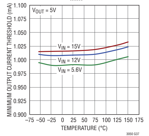
Minimum Output Current Threshold R_{I\text{MIN}} = 110k
