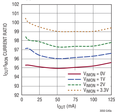
I_{\text{OUT}}/I_{\text{MON}} Current Ratio V_{\text{OUT}} = 3.3V , V_{\text{IN}} = 3.9V
