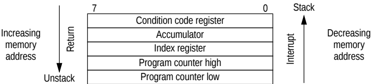
Figure 10-2 Stacking order
