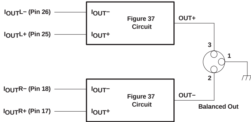
Figure 39. Measurement Circuit for Monoaural Mode
