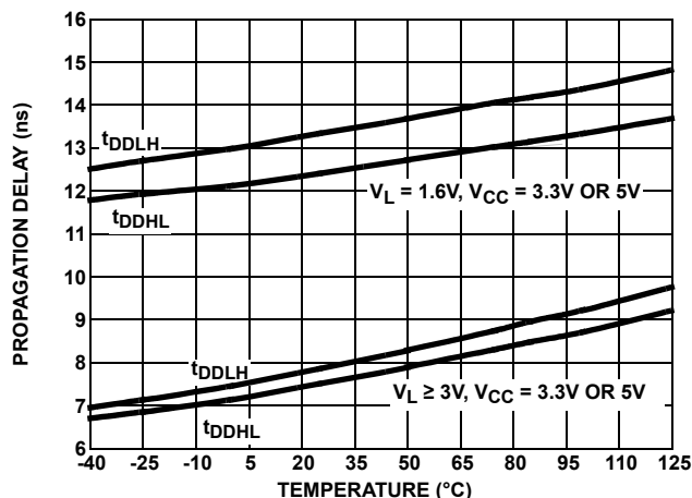
FIGURE 18. DRIVER DIFFERENTIAL PROPAGATION DELAY vs TEMPERATURE (ISL32172E, ISL32174E, ISL32179E, 32Mbps OPTION)
