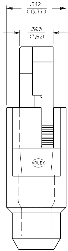
TERMINATED VIEWS
