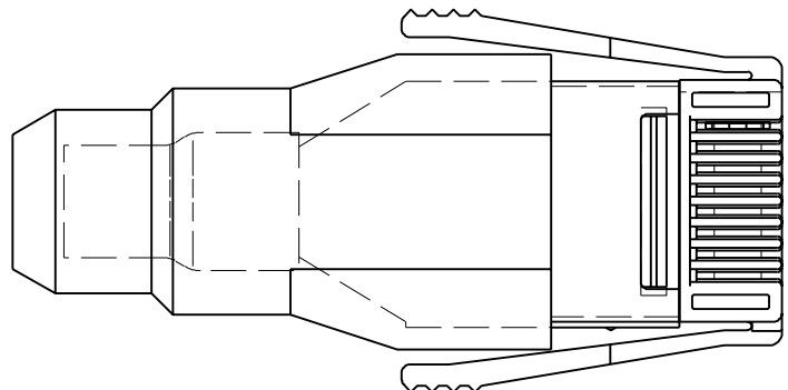
KEYING OPTION "1"
