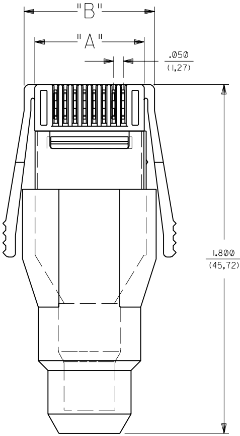
KEYING OPTION "1"
