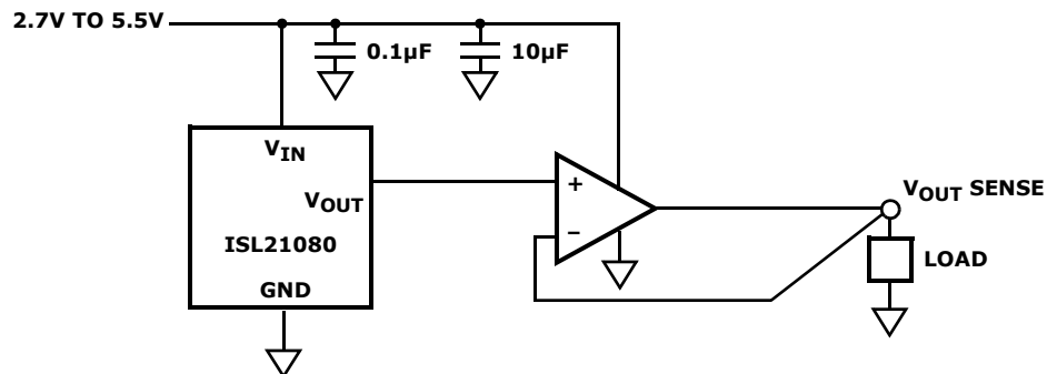
FIGURE 43. KELVIN SENSED LOAD
