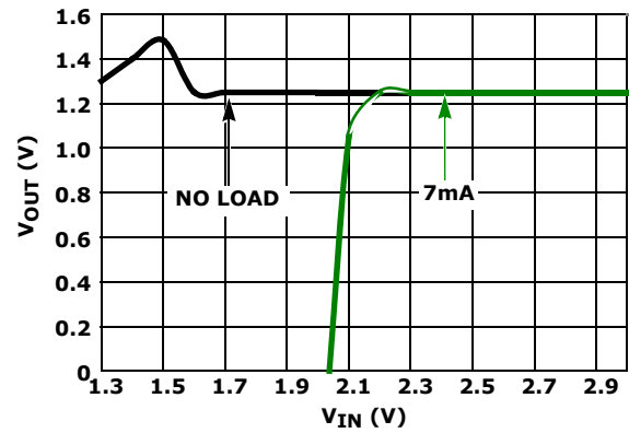
FIGURE 29. DROPOUT, ISL21080-12
