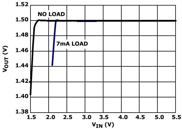
FIGURE 24. DROPOUT
