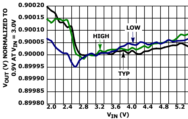
FIGURE 4. LINE REGULATION, 3 UNITS
