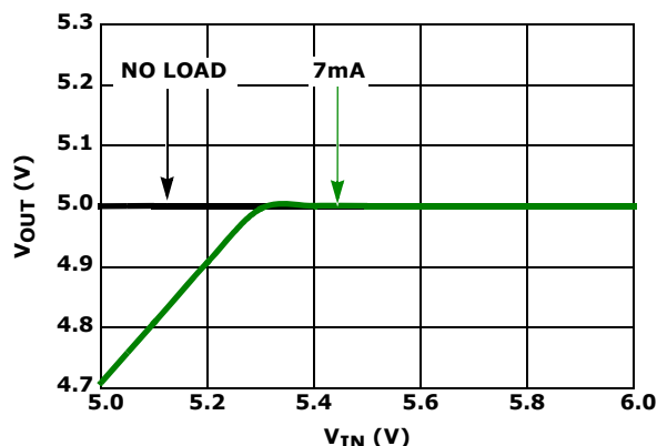
FIGURE 34. DROPOUT, ISL21080-50
