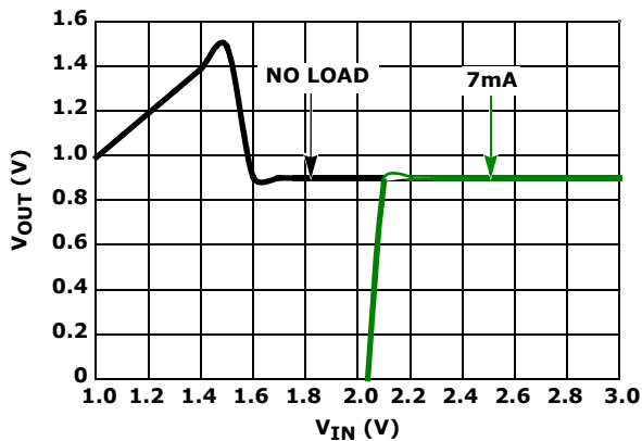
FIGURE 12. DROPOUT
