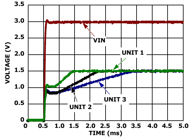
FIGURE 25. TURN-ON TIME
