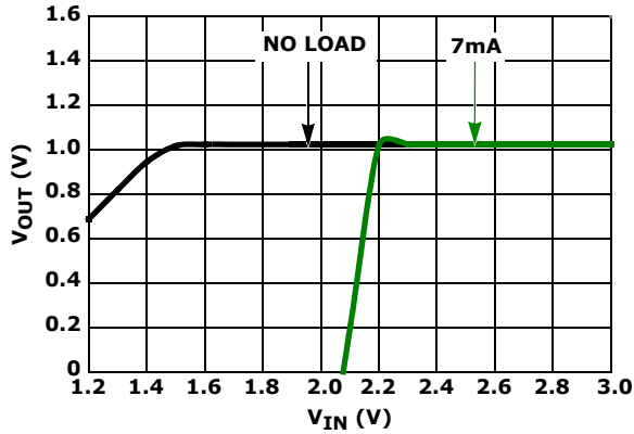
FIGURE 28. DROPOUT, ISL21080-10
