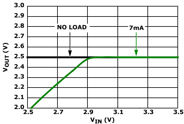
FIGURE 30. DROPOUT, ISL21080-25
