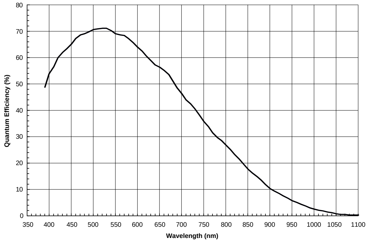
Figure 13. Quantum Efficiency – Monochrome Sensor
