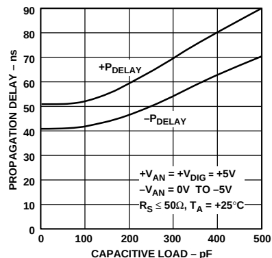
Figure 13. CMP402 Propagation Delay vs. Capacitive Load
