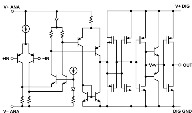
Figure 1. Simplified Schematic
