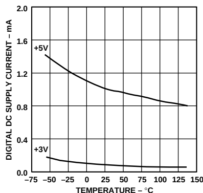
Figure 19. CMP402 Digital Supply Current vs. Temperature
