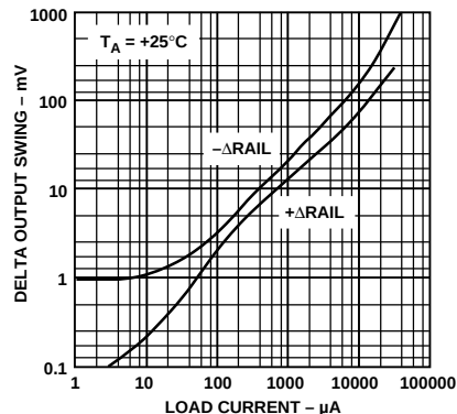
Figure 16. CMP401/CMP402 Delta Output Swing from Power Supplies vs. Load Current
