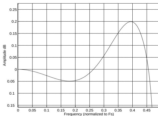
Figure 24. Passband Ripple
