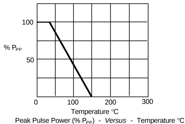
Figure 4 - Derating Curve
