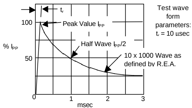
Figure 2 - Pulse Waveform
