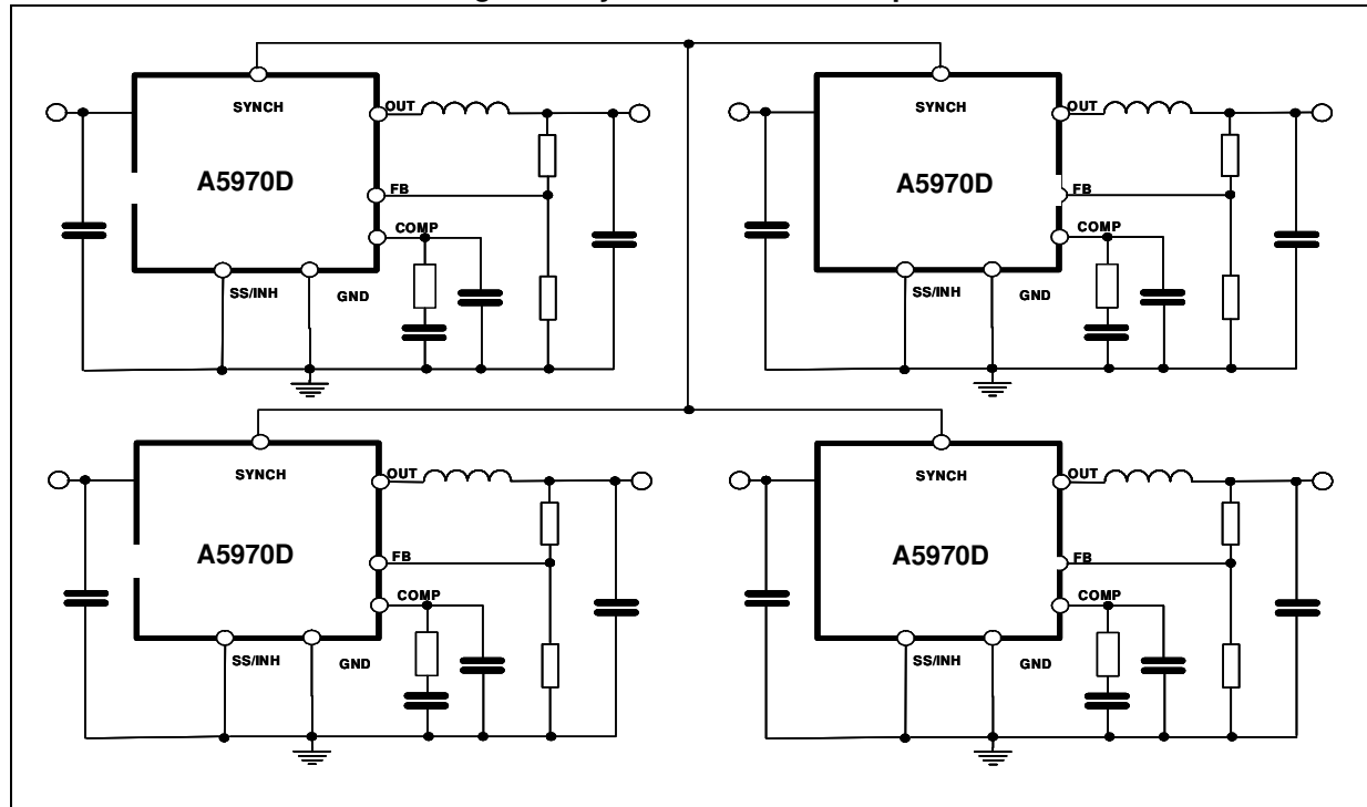
Figure 6. Synchronization example
