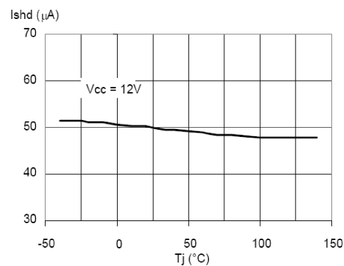
Figure 32. Shutdown current vs. junction temperature
