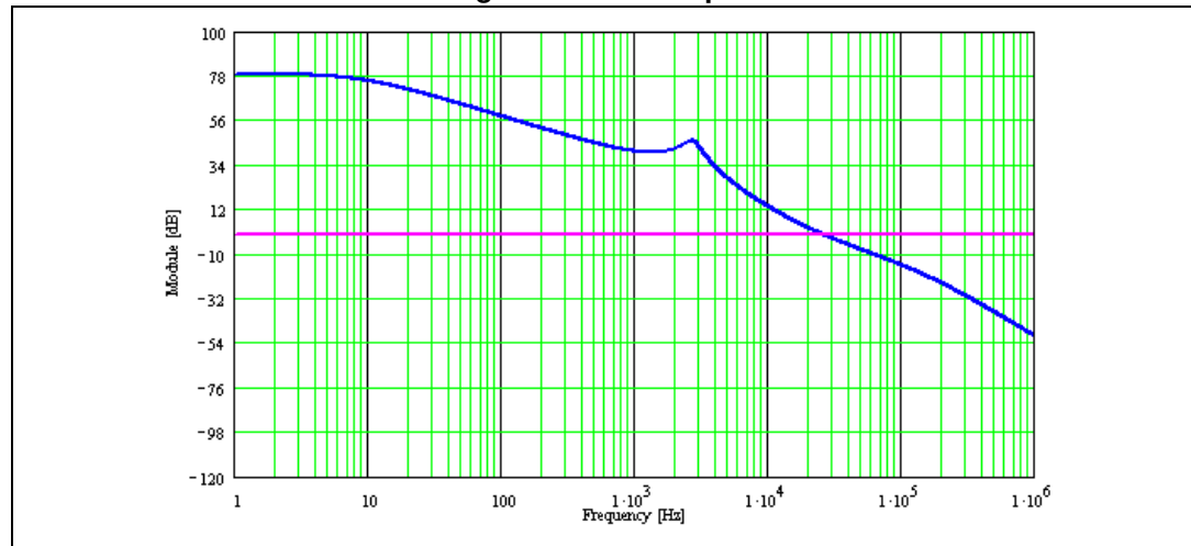
Figure 11. Module plot
