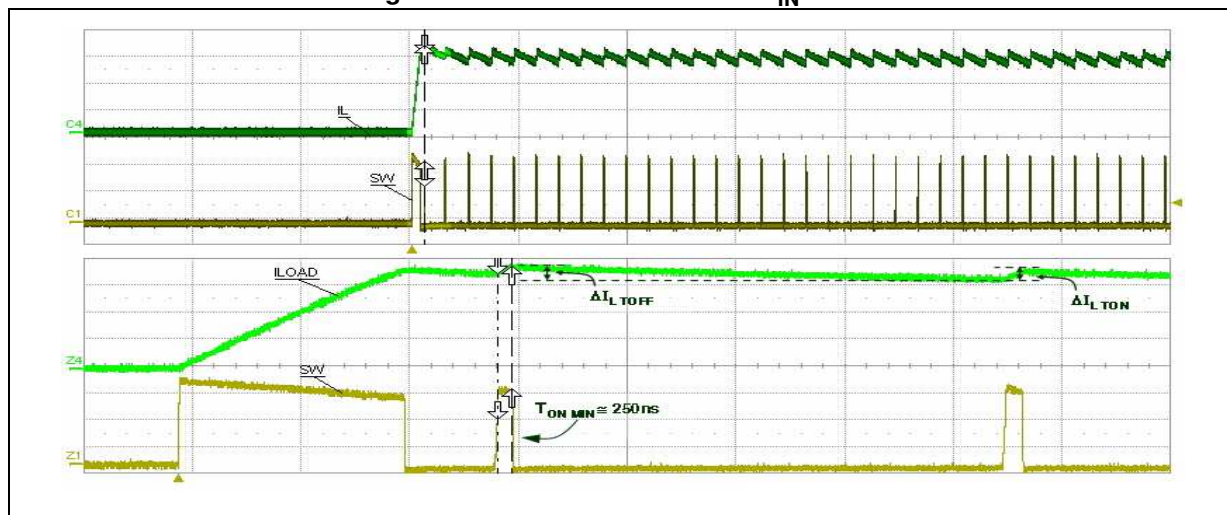
Figure 15. Short-circuit current V_{\text{IN}} = 12\text{ V}
