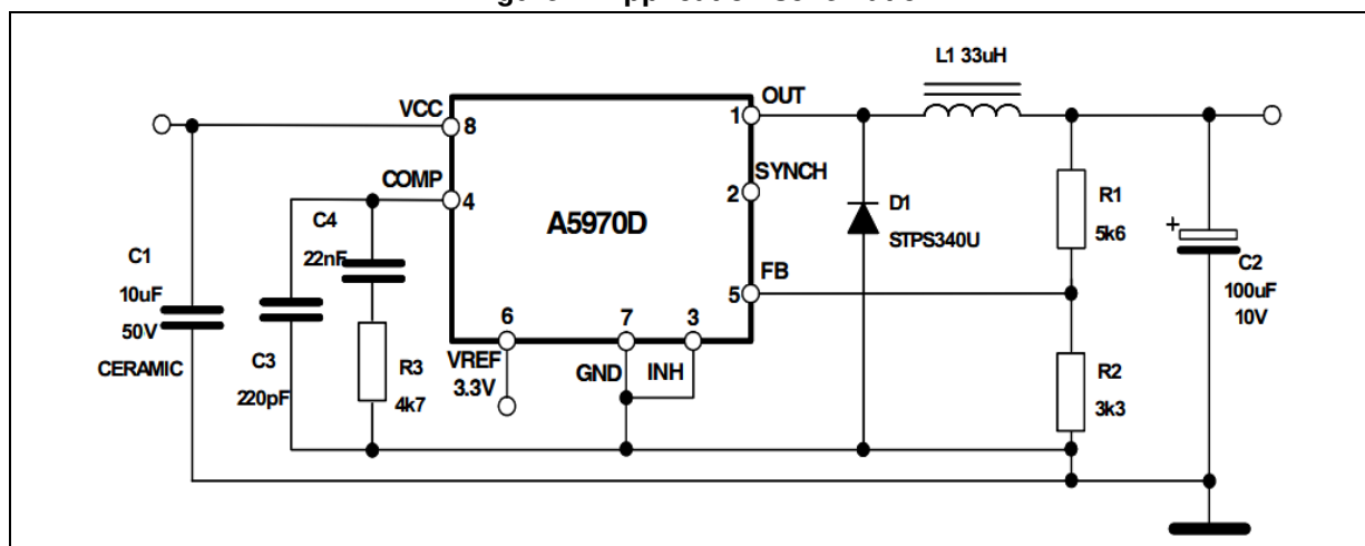
Figure 1. Application schematic
