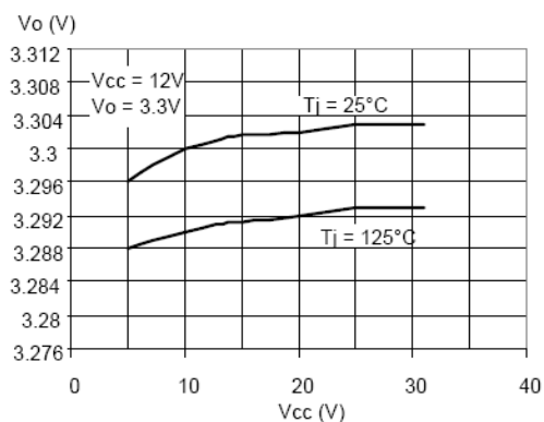
Figure 27. Line regulation
