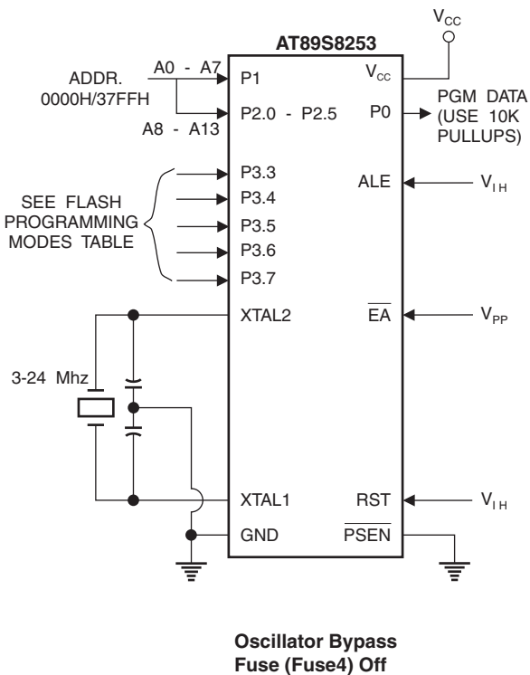
Figure 25-2. Verifying the Flash/EEPROM Memory (Parallel Mode)
