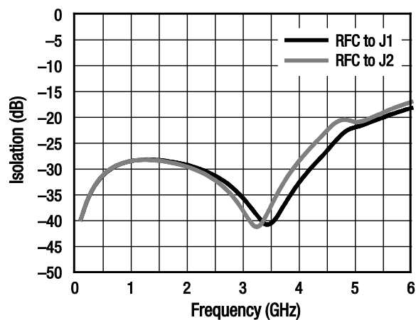
Figure 4. Typical Isolation
