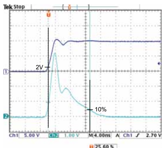
Figure 4: T_{OFF} at V_A = 10V
