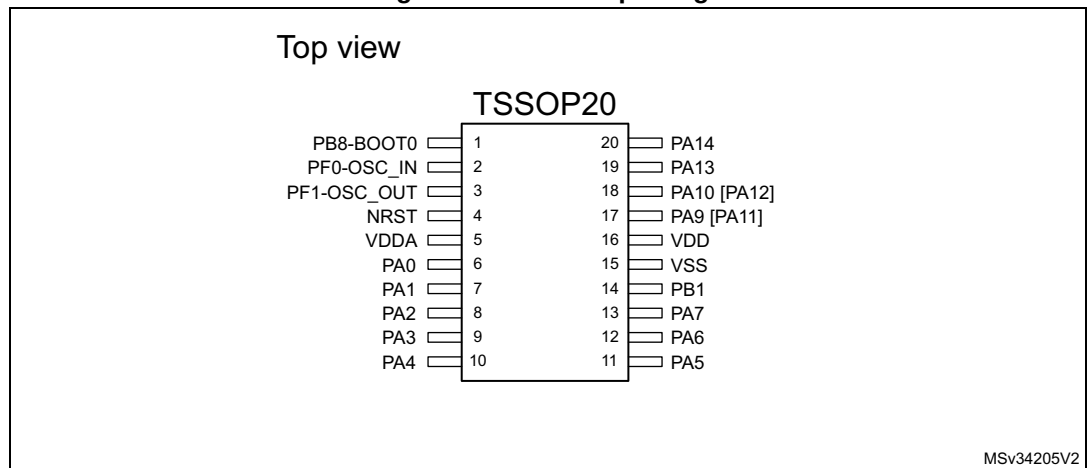
Figure 9. TSSOP20 package
