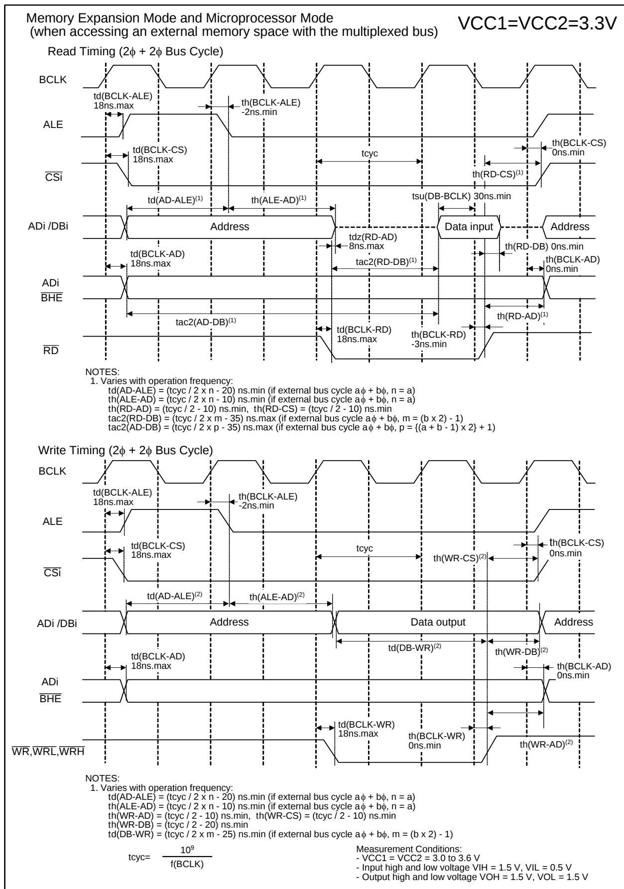
Figure 5.10 V_{CC1} = V_{CC2} = 3.3 \text{ V} Timing Diagram (4)
