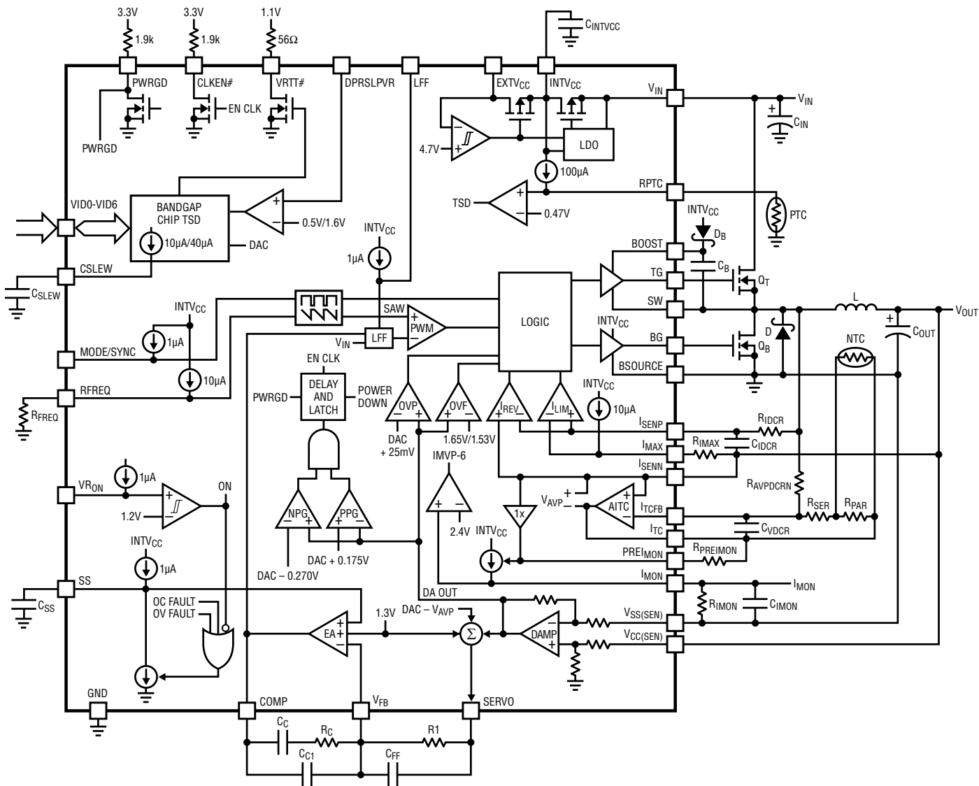
Figure 1. Functional Diagram
