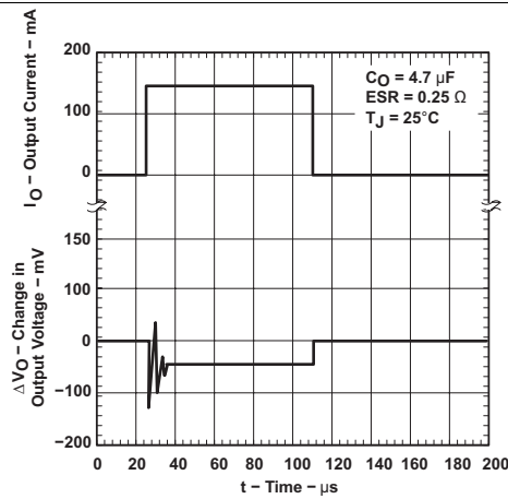
Figure 15. TPS76350-Q1 Load Transient Response
