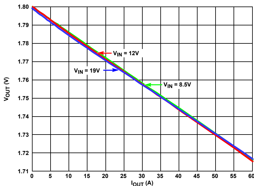
FIGURE 1. LOAD LINE REGULATION
