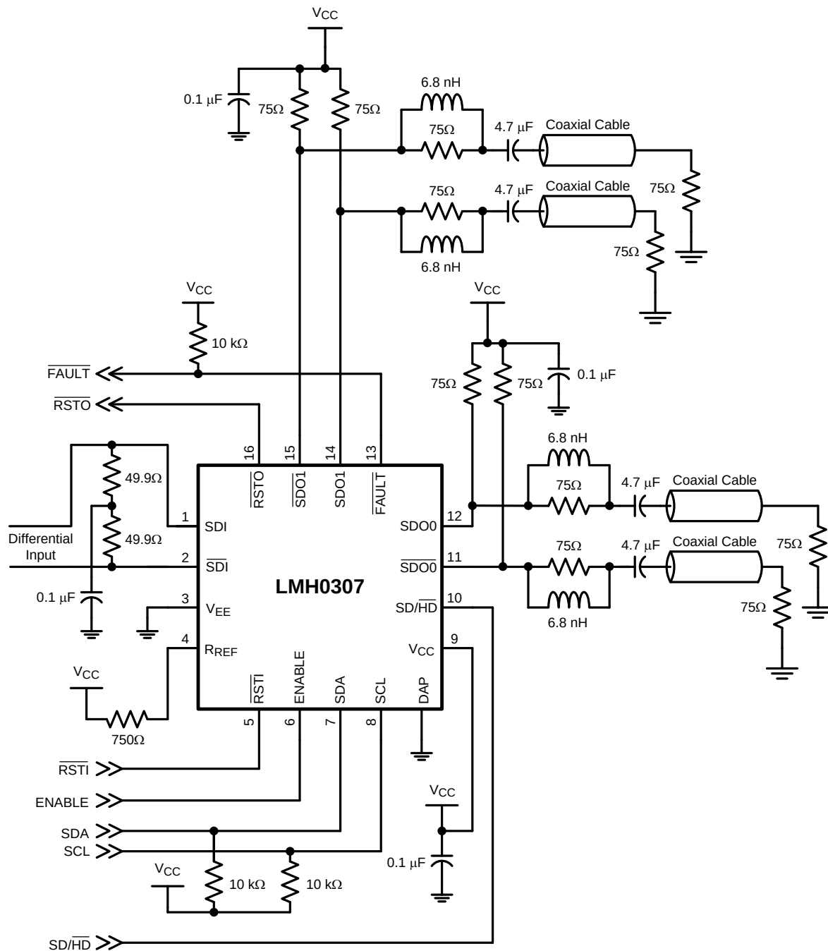
Figure 4. Application Circuit
