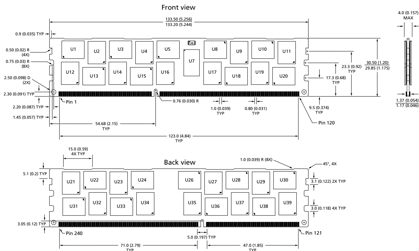
Figure 6: 240-Pin DDR3 RDIMM (R/C E2)
