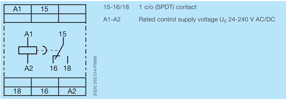
Connection diagram
