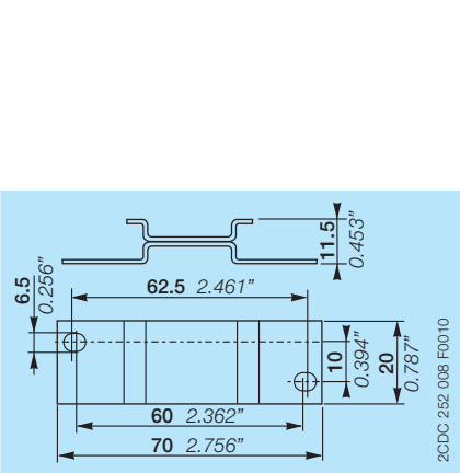
ADP.01 - Adapter for screw mounting
