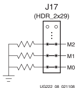
Figure 8: Default Configuration Mode Jumper Settings
