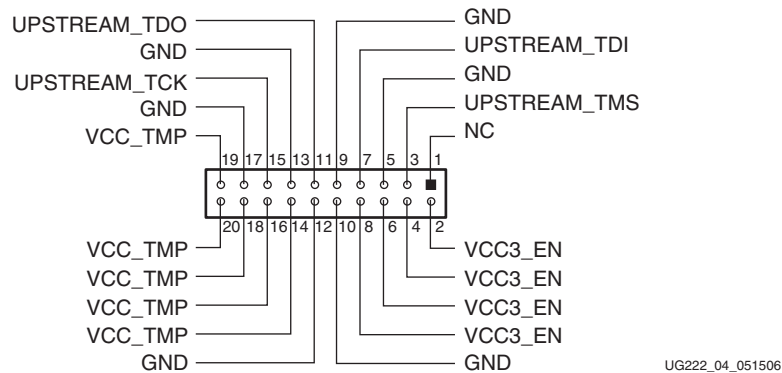
Figure 4: Upstream System ACE Interface Connector (20-Pin Female)
